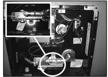
Fig 1: Water heater drain plug
