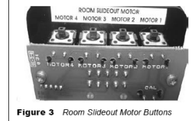
Figure 3 Room Slideout Motor Buttons
